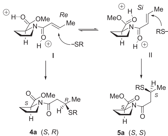
Scheme 3. Possible course of the transformation of 3 to 4a and 5a
