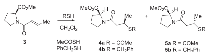
Scheme 2. Conjugate addition of thioacetic acid and \alpha -toluenethiol to compound 3 .
