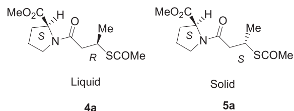
Fig. 1. Epimeric captopril derivatives.
