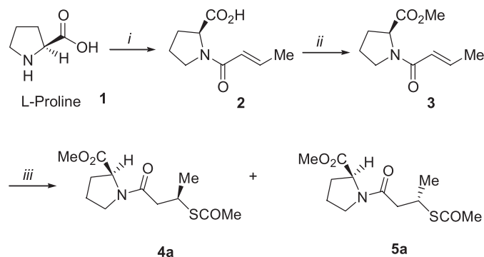
Scheme 1. i ) aq NaOH soln 5 %, \text{CH}_2\text{CH}=\text{CHCOCl} , ii ) \text{BF}_3 \cdot \text{MeOH} , reflux, 2h, iii ) \text{MeCOSH} , \text{CH}_2\text{Cl}_2 , -50^\circ\text{C} , 68 h.
