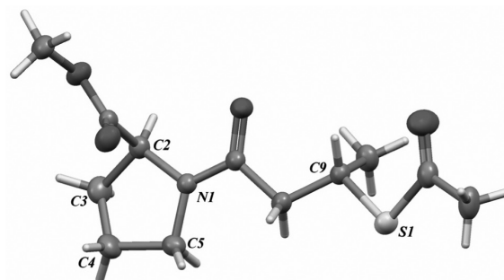
Fig. 2. Molecular structure of compound 5a . Displacement ellipsoids for non-H atoms are shown at the 30% probability level.
