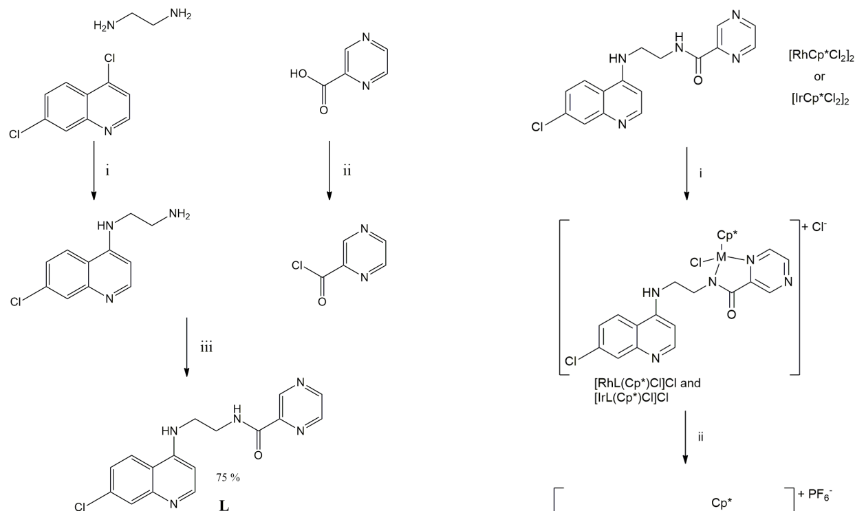
Scheme 1. Synthesis of L . Reagents and conditions: i) 130 °C, 8 h, neat. ii) SOCl 2 , reflux, followed by vacuum sublimation. iii) CH 2 Cl 2 , Et 3 N, 0 °C 3 h, RT overnight.
