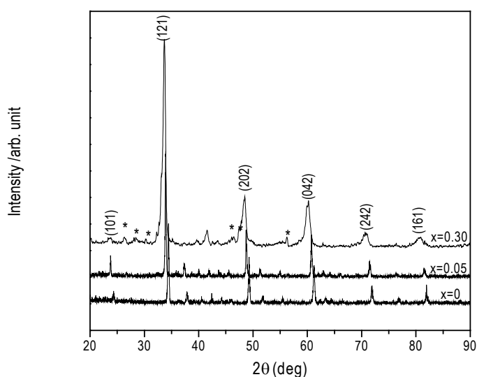
Figure 1. Powder X-ray diffraction pattern for \text{Eu}_x\text{Ca}_{1-x}\text{MnO}_3 (where x = 0, 0.05, 0.30 ). PDF-01-089-0666. (*) \text{Mn}_2\text{O}_4 -PDF-01-086-2337.
