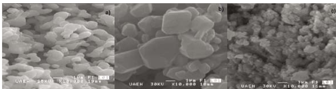
Figure 2. Scanning electron micrographs of \text{Eu}_x\text{Ca}_{1-x}\text{MnO}_3 manganite: a) x = 0 , b) x = 0.05 , c) x = 0.30 .
