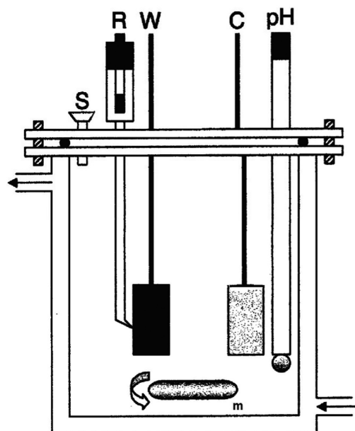
Fig. 3. Diagram of the one-compartment electrochemical cell used for studying anodic oxidation of \alpha zA: C, counter, R, reference, and W, working electrodes, respectively; pH electrode; S, sample holder; and m, magnetic stirrer.
